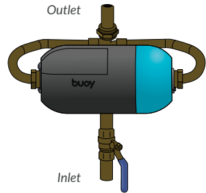
(Optional) waterhorn installation
